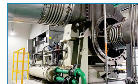
某电镍大循环项目硫酸镍蒸发浓缩装置蒸汽压缩机 Steam compressor for nickel sulfate evaporation and concentration unit of a certain electric nickel large cycle project
