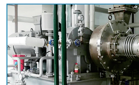
某焦化废水零排放项目蒸汽压缩机 Steam compressor for a zero discharge project of coking wastewater
